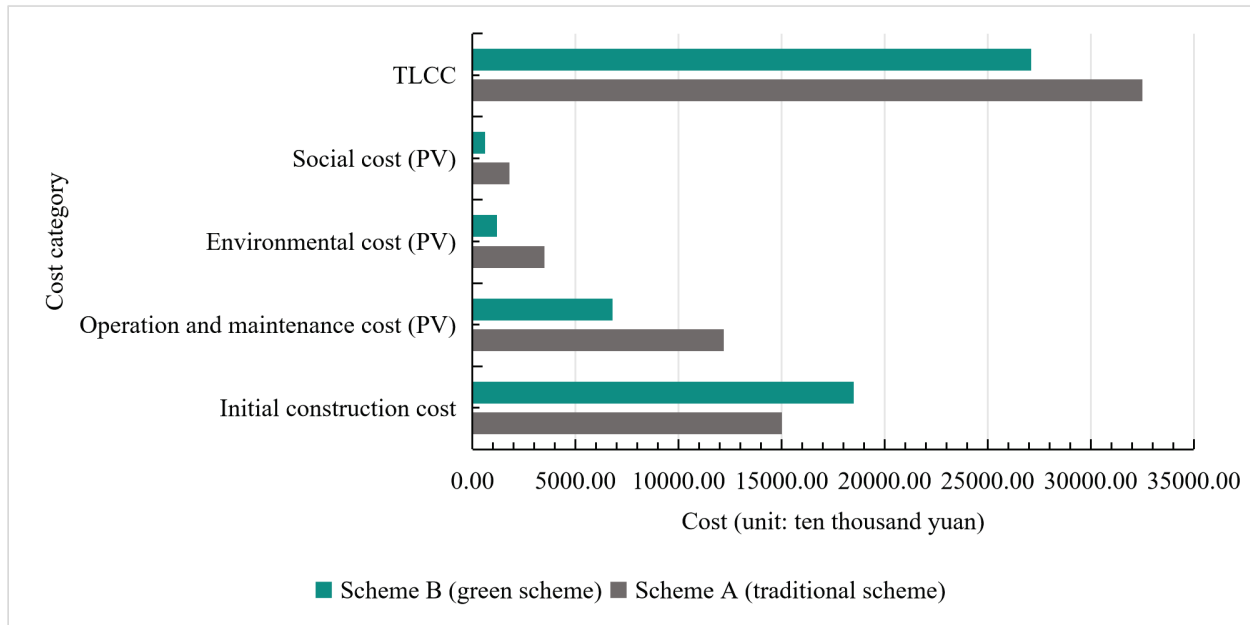
Figure 2 Comparison of LCC structure between two schemes
